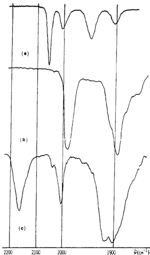
Figure 3. IR spectra of compounds 2 (a), 3 (b), and 4 (c) in the carbonyl stretching region. Solvent = CH 2 Cl 2 ( 2 ) and toluene ( 3 , 4 ).
