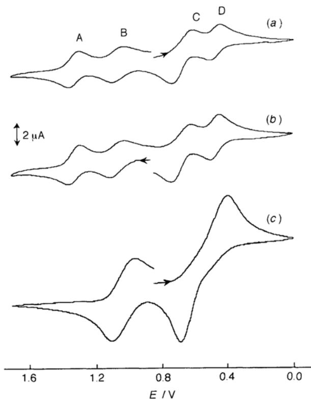
Fig. 2 Cyclic voltammetric studies of [(\text{Cp}^*\text{Mo})_2(\mu\text{-I})_4]\text{I}_3 , (a) and (b); \text{Bu}_4\text{NI}_3 , (c). Room temperature, Pt working electrode, Ag/AgCl reference electrode, \text{CH}_2\text{Cl}_2 solvent, \text{TBAPF}_6 supporting electrolyte.
