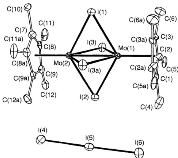
Fig. 1 Thermal ellipsoid diagram of [(\text{Cp}^*\text{Mo})_2(\mu\text{-I})_4]\text{I}_3 with the ions in their correct relative locations. Mo(1)–Mo(2), 2.718(3); all Mo–I, 2.78 \pm 0.01 ; Mo(1)–CNT(1), 2.012(6); Mo(2)–CNT(2), 1.993(6); I(4)–I(5), 2.919(5); I(5)–I(6), 2.905(5) Å. Mo–I–Mo, all 58.4 \pm 0.2 ; I(4)–I(5)–I(6), 178.7(2)^\circ ; (CNT = centre of cyclopentadienyl ring).
