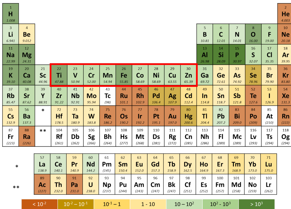
Figure 2: Abundance (in milligrams per kilogram of Earth's crust) of elements. First-row transition metals are more abundant than Ru, Os, Os, Ir or Au, commonly used in PDT. This review will present PS based on the metals framed in red.
