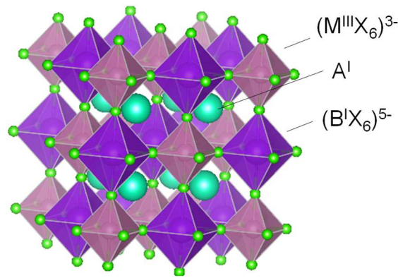
Fig. 1 View of the A'_2 B^I M^{III} X_6 double perovskite structure.
