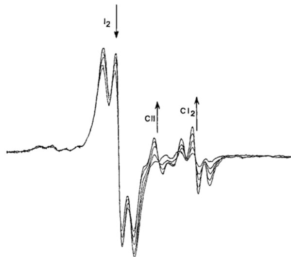
Figure 1. Representative EPR monitoring of the initial stages of a kinetic run for eq 2. T = 37.5 ^\circ\text{C} ; time interval = 4.5 h.
