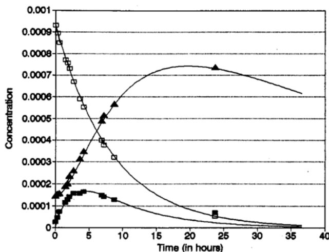
Figure 2. Representative variation of the concentration of CpMoI 2 (PMe 3 ) 2 (open squares), CpMoCl(PMe 3 ) 2 (dark squares), and CpMoCl 2 (PMe 3 ) 2 (dark triangles) with time, from the EPR monitoring of reaction 2. The data shown relate to run 15 of Table I.
