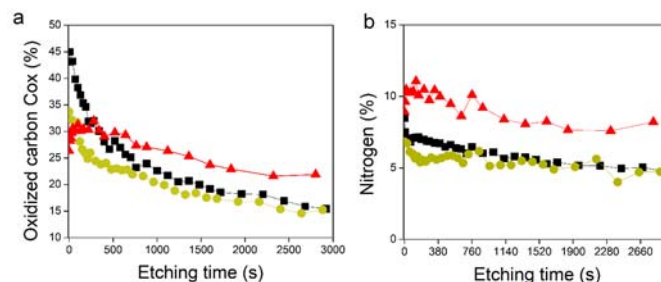
Fig. 8. Depth profiling of (a) C_{ox} and (b) nitrogen contributions the GOx/TA@AuNPs coating (red triangle), the GOx/TA@AuNPs drop-casted electrodeposited solution (yellow circle), and the GOx drop-casted solution (black square). The evolution is plotted as a function of the etching time by cluster argon bombardments at 8 KeV and 300 atoms.
