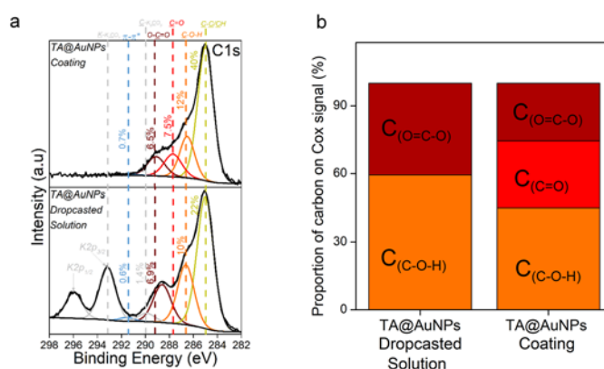
Fig. 6. (a) C 1s XPS spectra and (b) the relative contribution of each component in the oxidized organic carbon ( C_{ox} ) signal of the TA@AuNPs coating, obtained by electrodeposition of FcOH/TA@AuNPs and the TA@AuNPs drop-casted solution.
