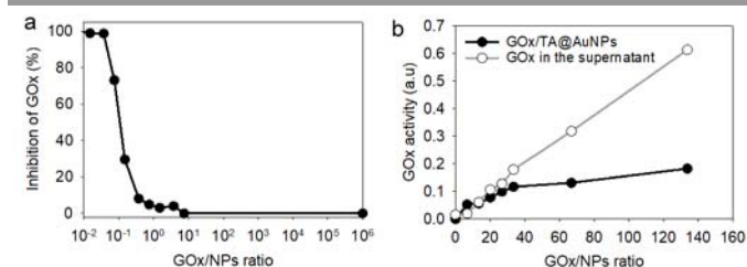
Fig. 3. GOx/TA@AuNPs activity (a) percentage of enzymatic inhibition in the presence of TA@AuNPs as a function of GOx/NPs ratio, in comparison to the same concentration of GOx in solution (b) enzymatic activity of rinsed GOx/TA@AuNPs, i.e. after centrifugation and redispersion in water, and the retrieved supernatant as a function of GOx/NPs ratio.
