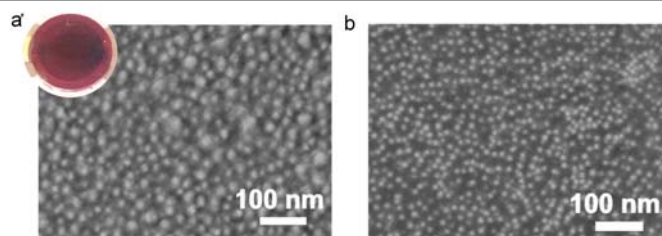
Fig. 5. SEM micrograph of the electrodeposited GOx/TA@AuNPs coating, with (a) secondary electron and (b) backscattered electron detector. GOx/TA@AuNPs coating was obtained from the electrodeposition of the FcOH/GOx/TA@AuNPs mixture. The inset is the photography of the gold QCM crystal after electrodeposition of the coating
