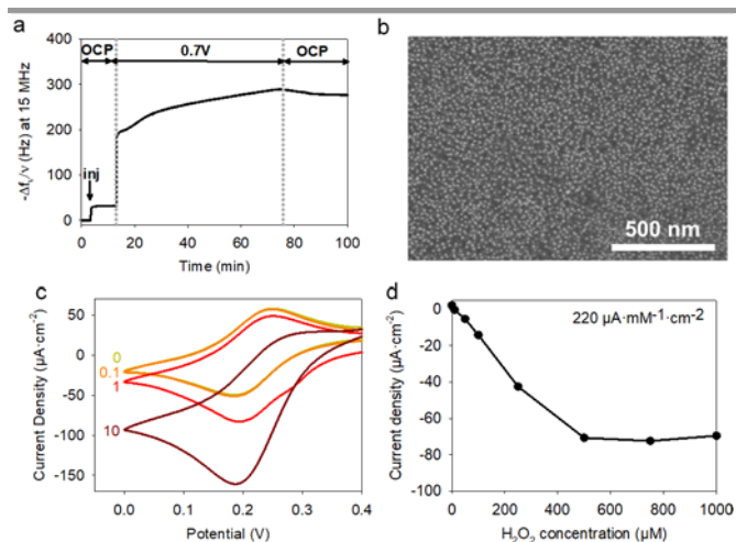
Fig. 11. HRP/TA@AuNPs coating: (a) Buildup with the evolution of the normalized frequency shift of FcOH/HRP/TA@AuNPs solution as a function of time during the application of 0.7 V (b) BSE-SEM micrograph of the coating, (c) Electrochemical reduction current, measured at 50 mV·s -1 , of 0 to 10 mM H 2 O 2 prepared in 0.5 mM FcOH/10 mM PBS and (d) Current density, measured at 0.19 V, as a function of H 2 O 2 concentration prepared in 0.1 mM FcOH/10 mM PBS.
