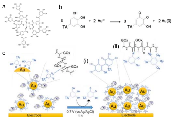
Scheme 1. (a) Chemical formulae of tannic acid (TA), (b) mechanism of TA@AuNPs synthesis by reduction of Au 3+ ions by TA in water. (c) Schematic representation of the electro-crosslinking of GOx/TA@AuNPs through electro-oxidation of gallol moieties of TA@AuNPs into quinone followed by the chemical reaction of quinone moieties with (i) gallol moieties of TA@AuNPs and (ii) free amino moieties of GOx through Michael addition and a Schiff's base condensation reaction.
