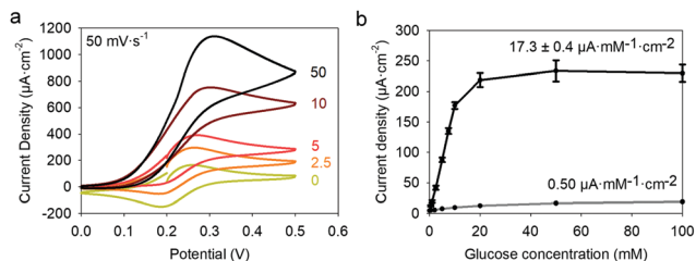
Fig. 9 (a) Cyclic voltammograms, performed at a scan rate of 50 \text{ mV s}^{-1} , of GOx/TA@AuNPs coating in contact with 0 to 100 mM of glucose solution prepared in 0.5 mM FcOH/10 mM PBS. (b) Average current density, measured at 0.25 V, as a function of the glucose concentration of GOx/TA@AuNPs (black curve) and GOx/TA (grey curve) coatings. The average and error bars of GOx/TA@AuNPs coatings were evaluated on six independent experiments.
