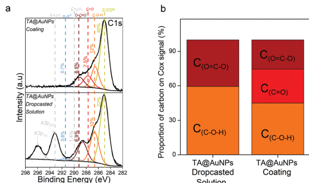
Fig. 6 (a) C 1s XPS spectra and (b) the relative contribution of each component in the oxidized organic carbon ( C_{ox} ) signal of the TA@AuNPs coating, obtained by electrodeposition of FcOH/TA@AuNPs and the TA@AuNPs drop-casted solution.
