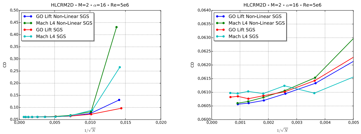
Figure 11. CRM-HL airfoil. Convergence of the total drag for the solution-adaptive process.
