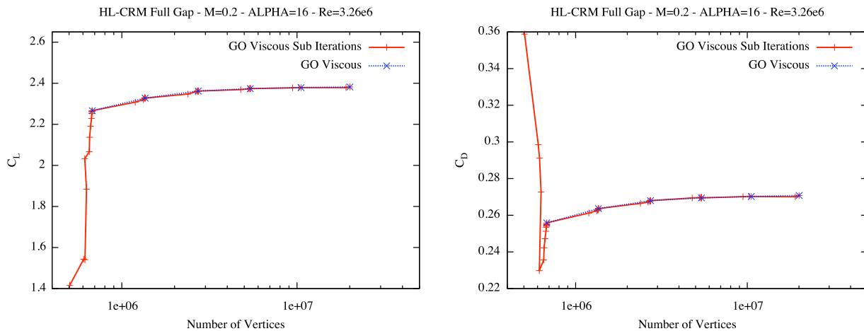
Figure 18. HLPW3 CRM-HL 16^\circ case. Convergence history of the total lift value C_L (left) and total drag value (right) for the viscous goal-oriented error estimate throughout the whole mesh-convergence analysis. In red, the convergence of the total lift at each complexity and, in blue, the global convergence of the total lift by retaining the final lift value for each complexity.
