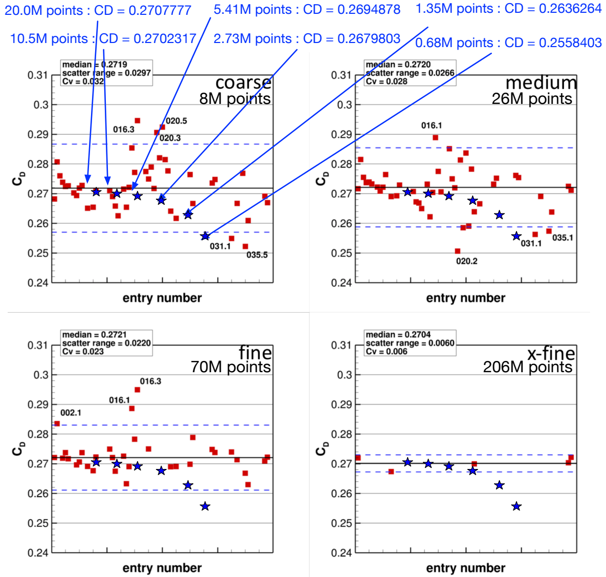
Figure 22. HLPW3 CRM-HL 16° case. Comparison of the drag prediction results obtained with the mesh-adaptive solution platform using the viscous goal-oriented error estimate (blue stars) with respect to all the HLPW3 results (red squares) obtained on the coarse (top left), medium (top right), fine (bottom left) and x-fine (bottom right) meshes.
