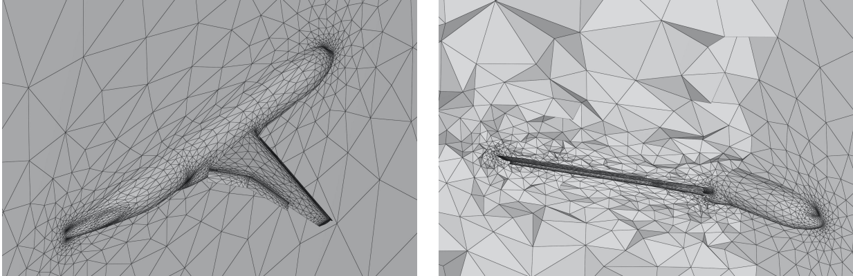
Figure 17. HLPW3 CRM-HL 16^\circ case. Initial coarse and clearly unresolved mesh only composed of 51 314 vertices, 265 482 tetrahedra and 26 692 triangles on the surface.
