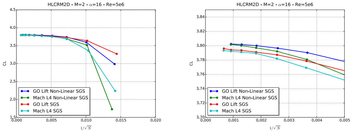
Figure 10. CRM-HL airfoil. Convergence of the total lift for the solution-adaptive process.
