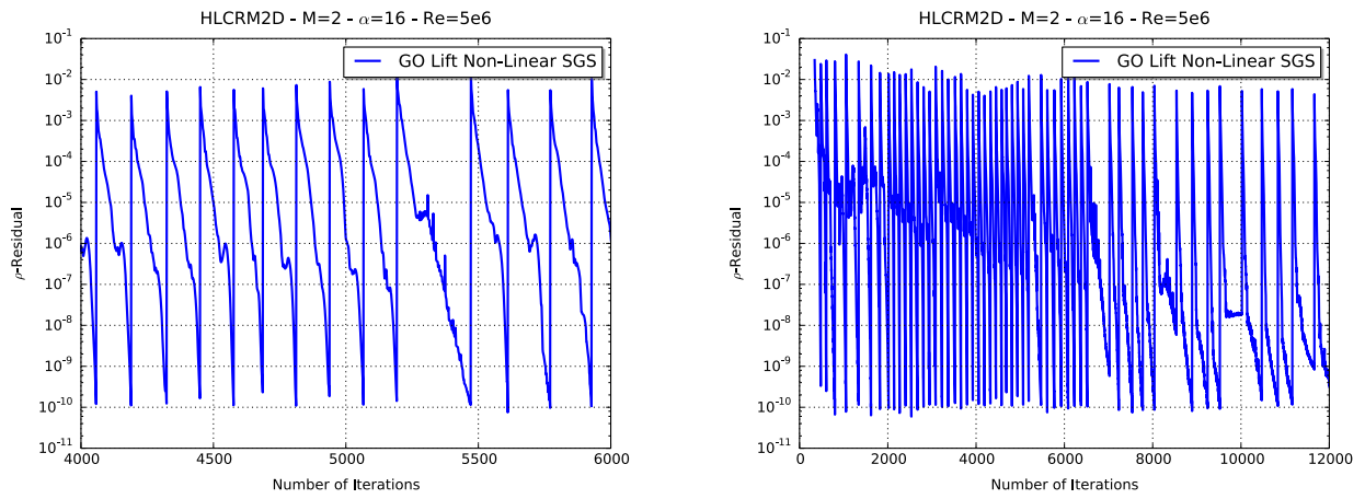
Figure 9. CRM-HL airfoil. History of the \rho -residual throughout the whole solution adaptive process. Each increases of the residual corresponds to a new run on a new adapted mesh.
