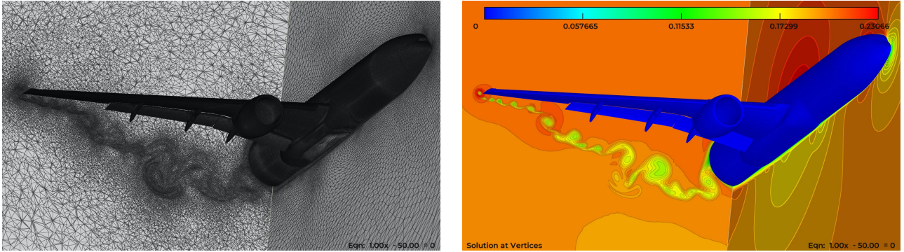
Figure 23. HLPW4 CRM-HL 7^\circ case. Adapted mesh composed of 20M vertices and associated solution field (local Mach number) for the cut plane x = 50 .
