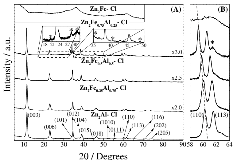
Figure 2. (A) XRD patterns of the \text{Zn}_2\text{Fe}_y\text{Al}_{(1-y)}\text{-Cl} samples; (*) indicates the presence of \text{Zn}(\text{OH})_2 and \text{ZnO} phases. (B) Magnification in the 58 – 64 ( 2\theta ) range; the dotted line shows the shift of the (110) reflection to the left as y increases.
