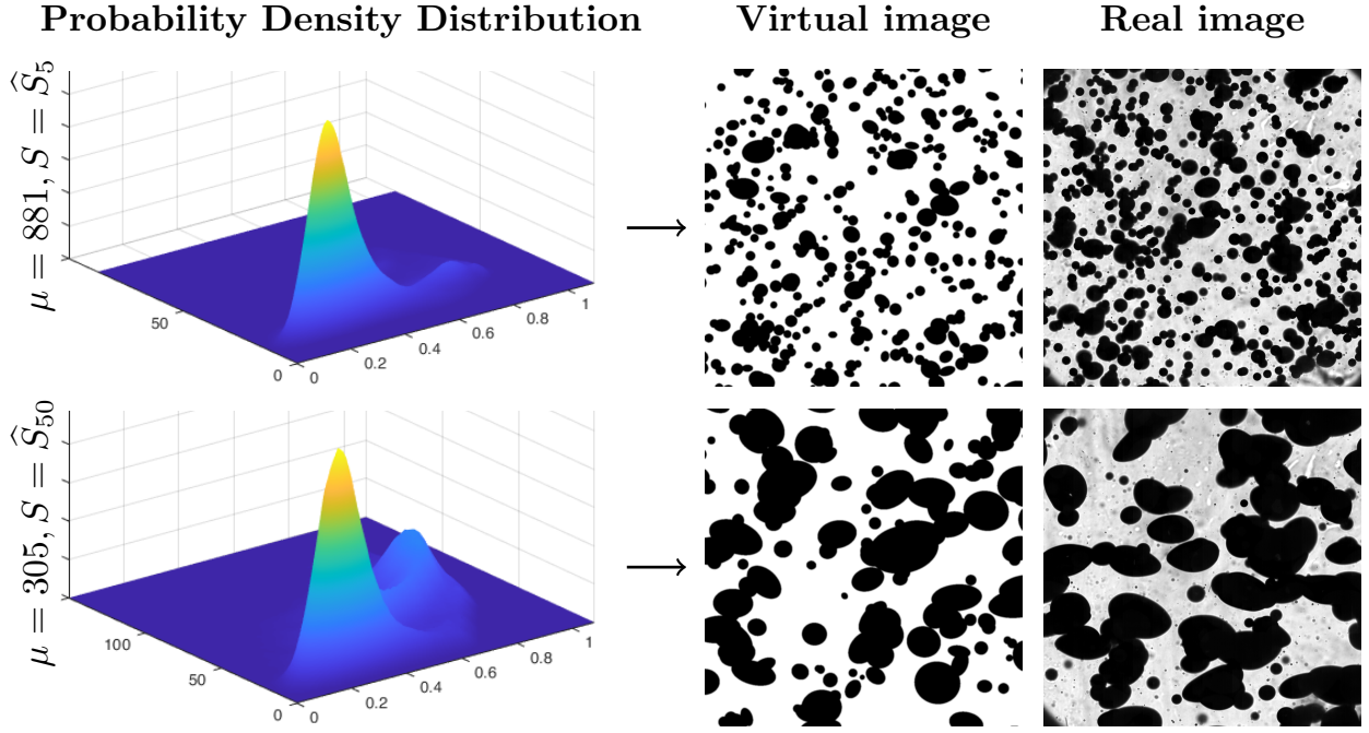
Fig. 7: Probability density functions reconstructed with the data obtained from the ellipse detection algorithm for \nu = 5 (top) and \nu = 50 (bottom) and comparison of the virtual and real images.
