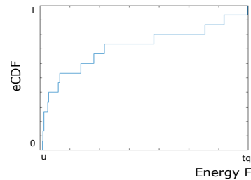
Fig. 2: Empirical cumulative distribution function of \mathbb{U} samples
