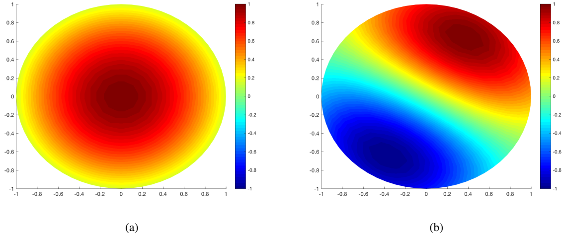
Figure 9: Mode shapes of (a) L(0,1) and (b) F(1,1) in a solid aluminium cylinder 1 m long and 14 mm in diameter for f = 100 kHz.
