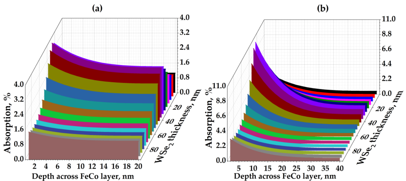
Figure 5. Calculated dependences of the optical absorption on the depth across the FM layer and on the thickness of the TMD layer in (a) \text{FeCo}_{20}/\text{WSe}_2 and (b) \text{FeCo}_{40}/\text{WSe}_2 .
