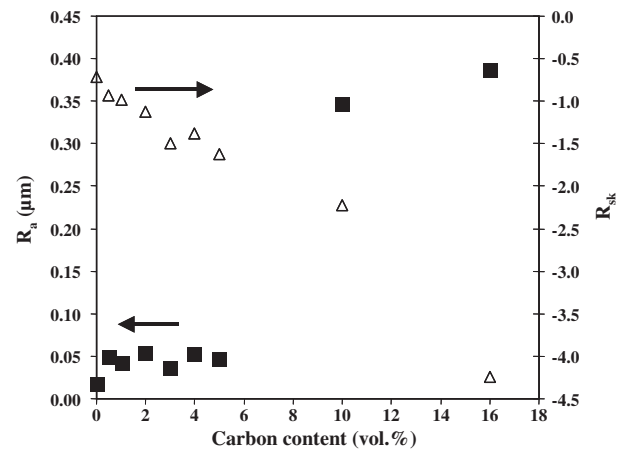
Fig. 8 – Calculated roughness ( R_a ) (a) and calculated skewness ( R_{sk} ) versus the carbon content (b). See text for details.
