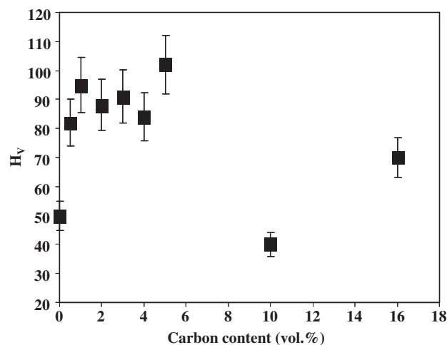
Fig. 9 – Vickers microhardness versus carbon content.
