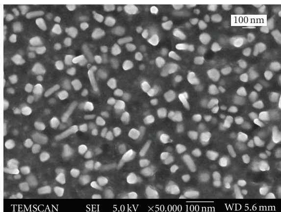
FIGURE 2: FEG SEM micrograph of the copper particles produced by heat treatment of the OP1 oxalate under N_2 at 280^\circ C .
