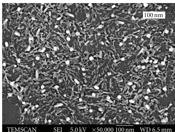
FIGURE 3: FEG SEM micrograph of the partially decomposed OP2 oxalate reduced under hydrogen at 200^\circ C for 5 hours.
