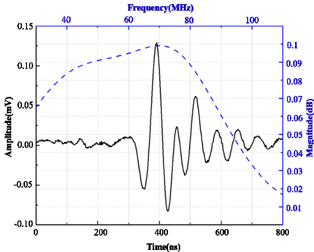
Fig. 8 Pulse-echo signal testing and spectrum analysis of the transducer
