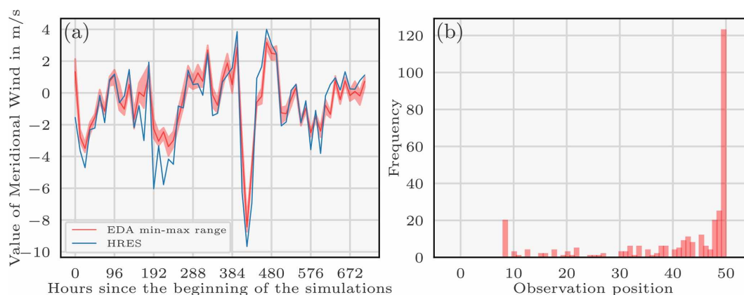
Figure 6. Evolution of the meridional wind of the HRES and EDA meteorologies for a random location in Europe since the beginning of the simulations. The red curve represents the mean of the meridional wind EDA members with the space between the minimum and maximum values (a). Rank histogram: comparison between the ^{106}\text{Ru} observations and the reference predictions of the enhanced ensemble (b).
