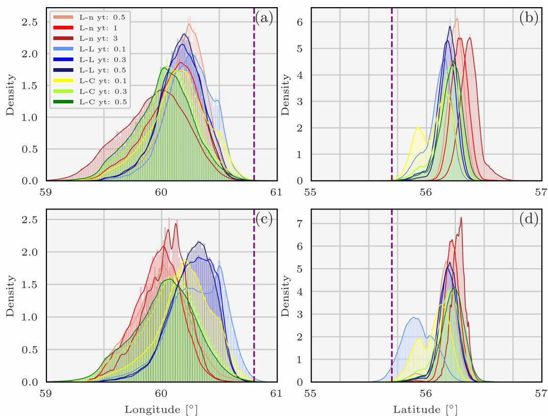
Figure 4. Pdfs of the coordinates describing the ^{106}\text{Ru} source sampled using the parallel tempering method and the observation-sorting algorithm and for various likelihoods in two scenarios: longitude without (a) and with observation spatial clustering in nine clusters (c) and latitude without (b) and with (d). L-L means log-Laplace, L-n means log-normal, L-C means log-Cauchy, and y_t is the likelihood threshold. The purple vertical bars represent the coordinates of the Mayak nuclear complex.
