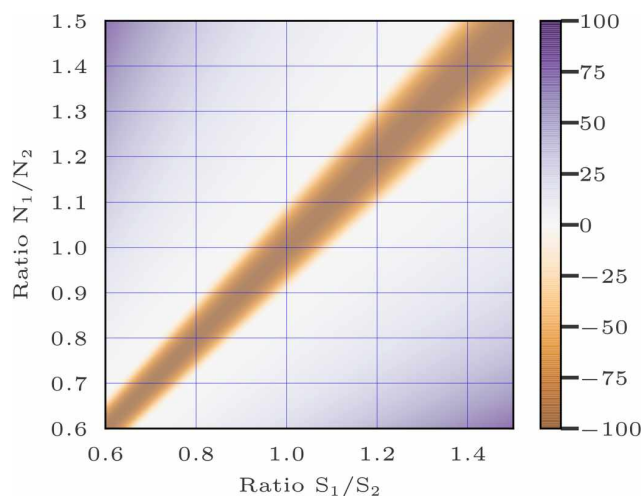
Figure B1. \text{AIC}(0) - \text{AIC}(d) with negative values multiplied by 100 to be more visible. Negative values indicate the cases where the model (0) with one variable is preferable. Positive values indicate the cases where the model ( d ) with two variables is preferable. On the x axis is the ratio between the likelihoods S_1 and S_2 linked to variables 1 and 2, respectively, of the model ( d ). On the y axis is the ratio between the numbers of observations N_1 and N_2 linked to variables 1 and 2, respectively, of the model ( d ).
