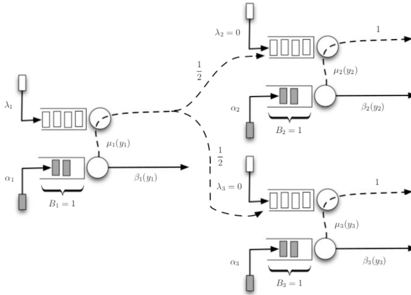
Fig. 2. Three-blocks EPN.
