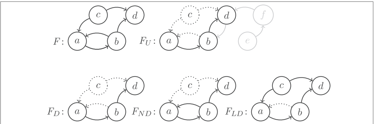
Figure 3: An update and different kinds of deletions
