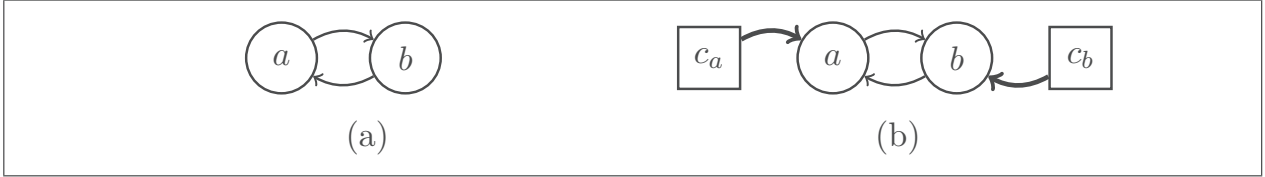
Figure 10: Transforming an AF into a CAF
