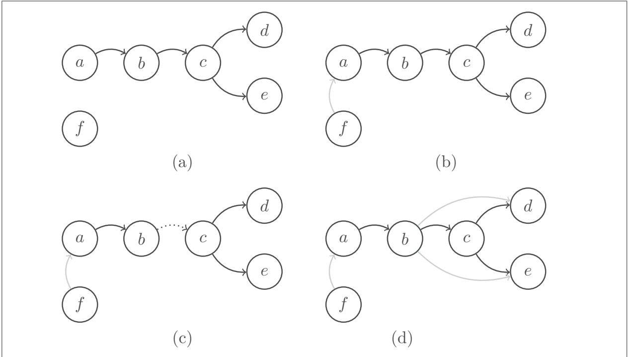
Figure 8: Example candidate AFs for Algorithm 1
