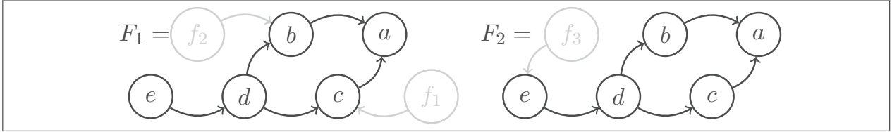
Figure 7: An example of (non-)minimal change
