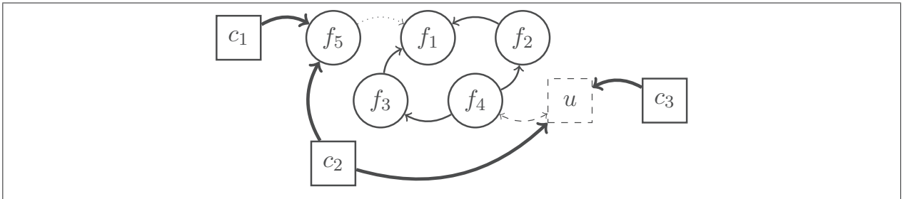
Figure 9: An example of control argumentation framework
