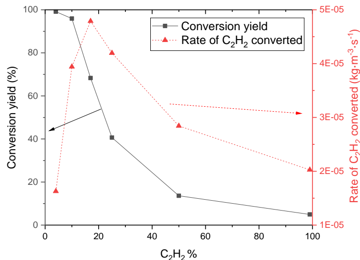
Figure 5: Acetylene conversion yield and rate of C_2H_2 converted as a function of C_2H_2\% .
