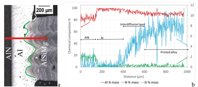
Fig. 5. (a) Interface images using backscattered electrons and (b) EDX detected element distribution on the red line on the interface image (from left to right).
