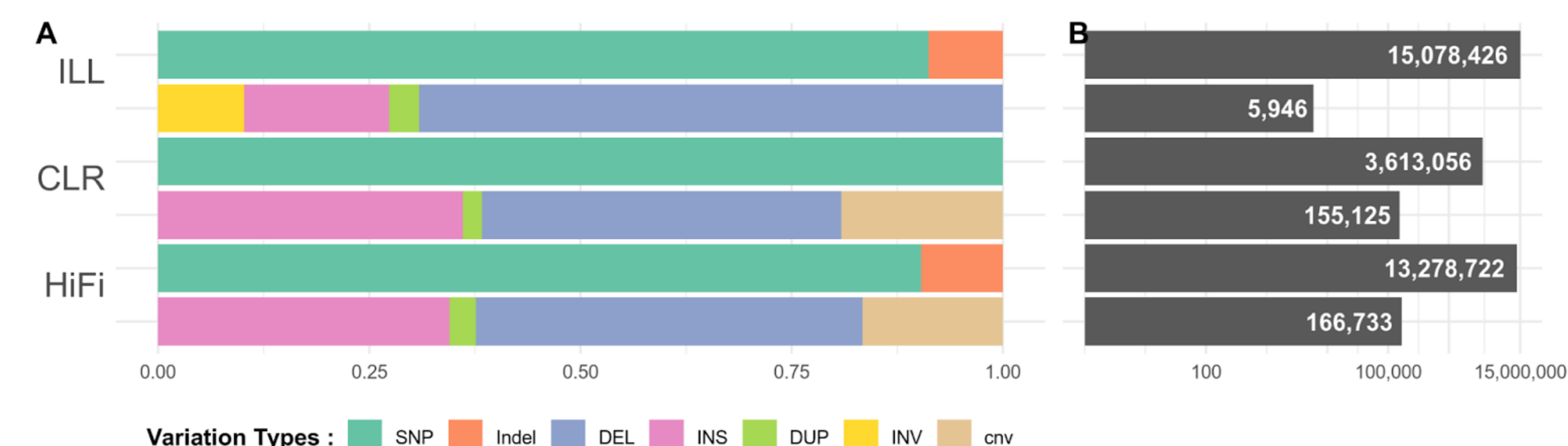
Figure 2 : Variant calling comparison between sequencing technologies on Maize1.
