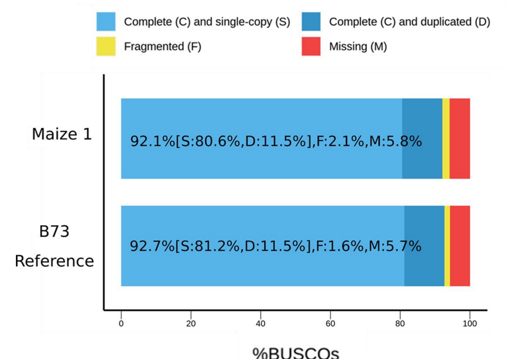
Figure 4 : Busco (v4.0.2) statistics of Maize 1 assembly versus B73 reference sequence.
