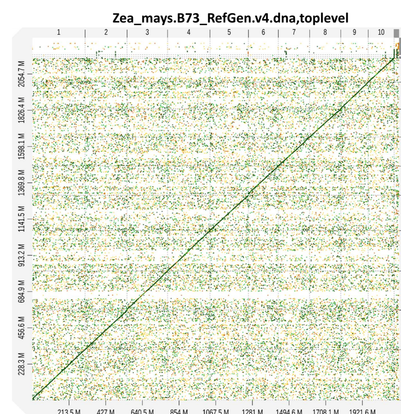
Figure 3 : Alignment results of Maize1 assembly to the B73 reference sequence.
