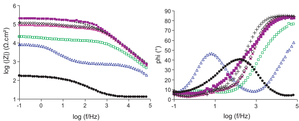
Fig. 12. Bode representation plotted after 1 h of immersion of zinc substrate in a 0.5 M \text{Na}_2\text{SO}_4 solution ( \bullet ), 80°C dried sample ( \Delta ), 110°C ( \square ), 130°C ( \blacktriangle ), 150°C ( \diamond ), 180°C ( \blacksquare ) and (+) for standard dried sample.
