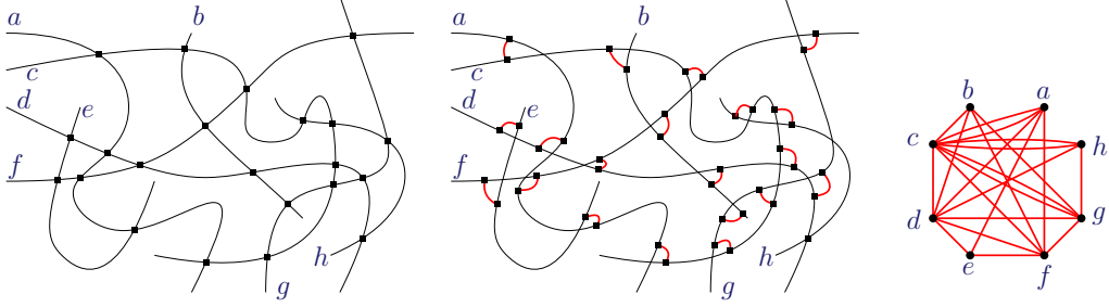
Figure 4: An example of the proof of Proposition 12 . In the leftmost figure we see a collection of lines in the plane \mathcal{L} = \{L_1, \dots, L_k\} whose intersection graph G_{\mathcal{L}} is depicted in the rightmost figure and has maximum edge degree 9 because of line c that meets other lines in 9 points, therefore G_{\mathcal{L}} \in \mathcal{S}_9 . To see why G_{\mathcal{L}} \in \mathcal{P}^{(1,9)} , one may see the leftmost figure are a planar graph P \in \mathcal{P} where vertices of degree 1 are discarded. The vertices of this planar graph can be seen as the result of the contraction of the red edges (seen as subgraphs of diameter 1) in the graph J in the middle, i.e., P \leq^{(1)} J . Finally, the intersection graph G_{\mathcal{L}} can be seen as a result of the contraction in J of each one of the paths, on at most 9 vertices, to a single vertex. Therefore G_{\mathcal{L}} \leq^9 J , hence G_{\mathcal{L}} belongs in the (1, 9) -extension of planar graphs.
