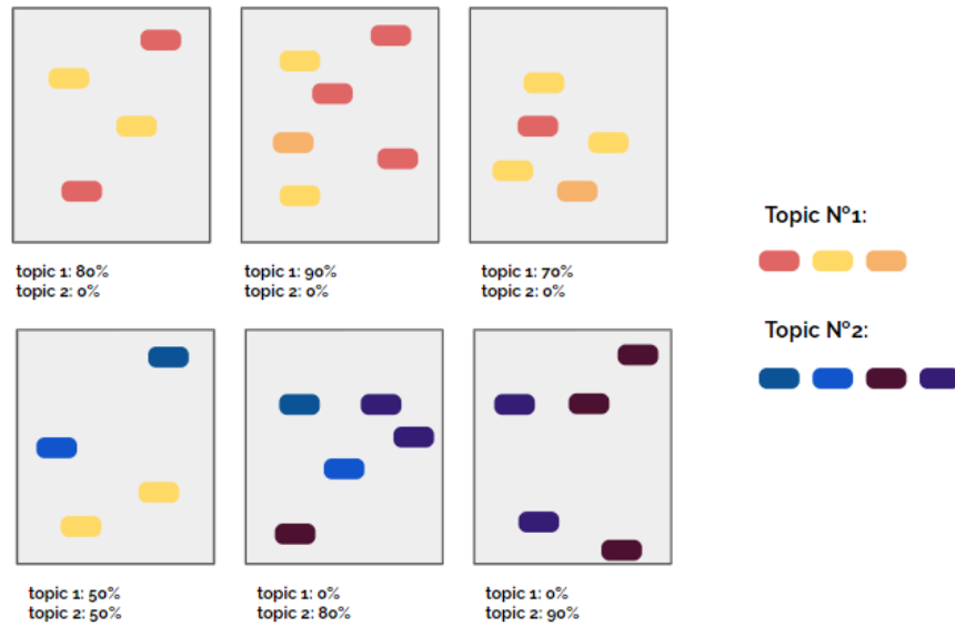
Fig. 2. On this Figure the scheme of the LDA algorithm is presented. On the example, two topics (on the right) are extracted from the six textual documents (on the left) containing the set of words (different words are shown in different colours). Based on words frequency and relevancy within the document the topic relevance to the document is calculated.
