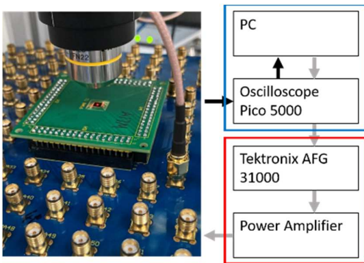
Fig. 3. LDV setup for characterizing the PMUT performance.
