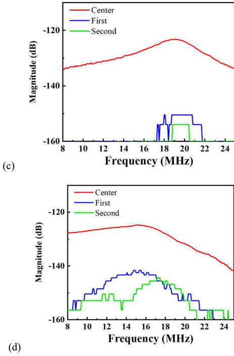
Fig. 5. The crosstalk response of the C-PMUT and B-PMUT under air and water load respectively. (a) The response of C-PMUT with air load. (b) The response of C-PMUT with water load. (c) The response of B-PMUT with air load. (d) The response of B-PMUT with water load.
