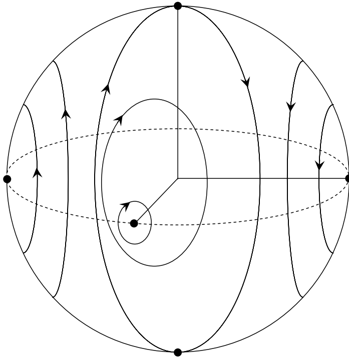
FIGURE 4. The phase portrait on the sphere \mathbb{S}^2 of the infinity. There are only drawn the orbits contained in the closure of the local chart U_1 .
