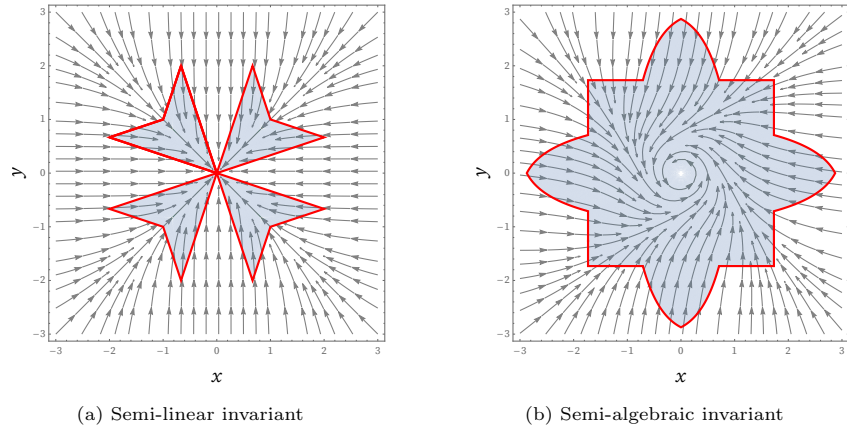
Figure 2: Positive invariants
