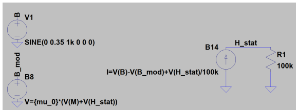
Fig. 2. Inversion of the EB model thanks to [7].
