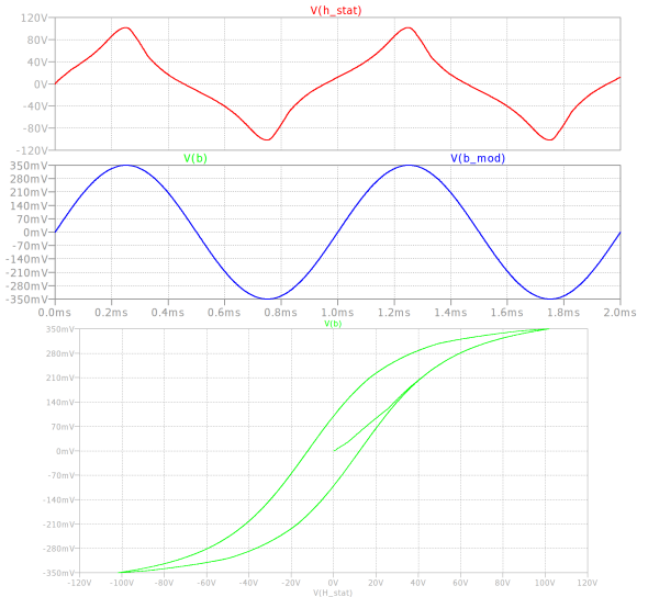
Fig. 3. Temporal waveforms (up) and corresponding BH loop (down) loop for \hat{B} = 0.35 T, f = 1 kHz. (units scale 1\text{T}=1\text{V} for V(B) ; 1\text{V}=1 A/m for V(H_{stat}) )
