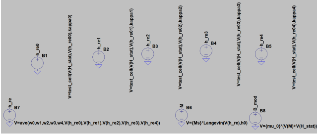
Fig. 1. Example of Behavioural Voltage (BV) sources.
