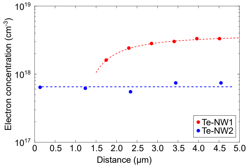
Figure 4. Spatial dependence of the electron concentration along the axis of the NW grown at 640 °C (Te-NW1, red) and at 620 °C (Te-NW2, blue). The bottom of the NW is at 0 \mu\text{m} . The dotted lines serve as guides to the eye.
