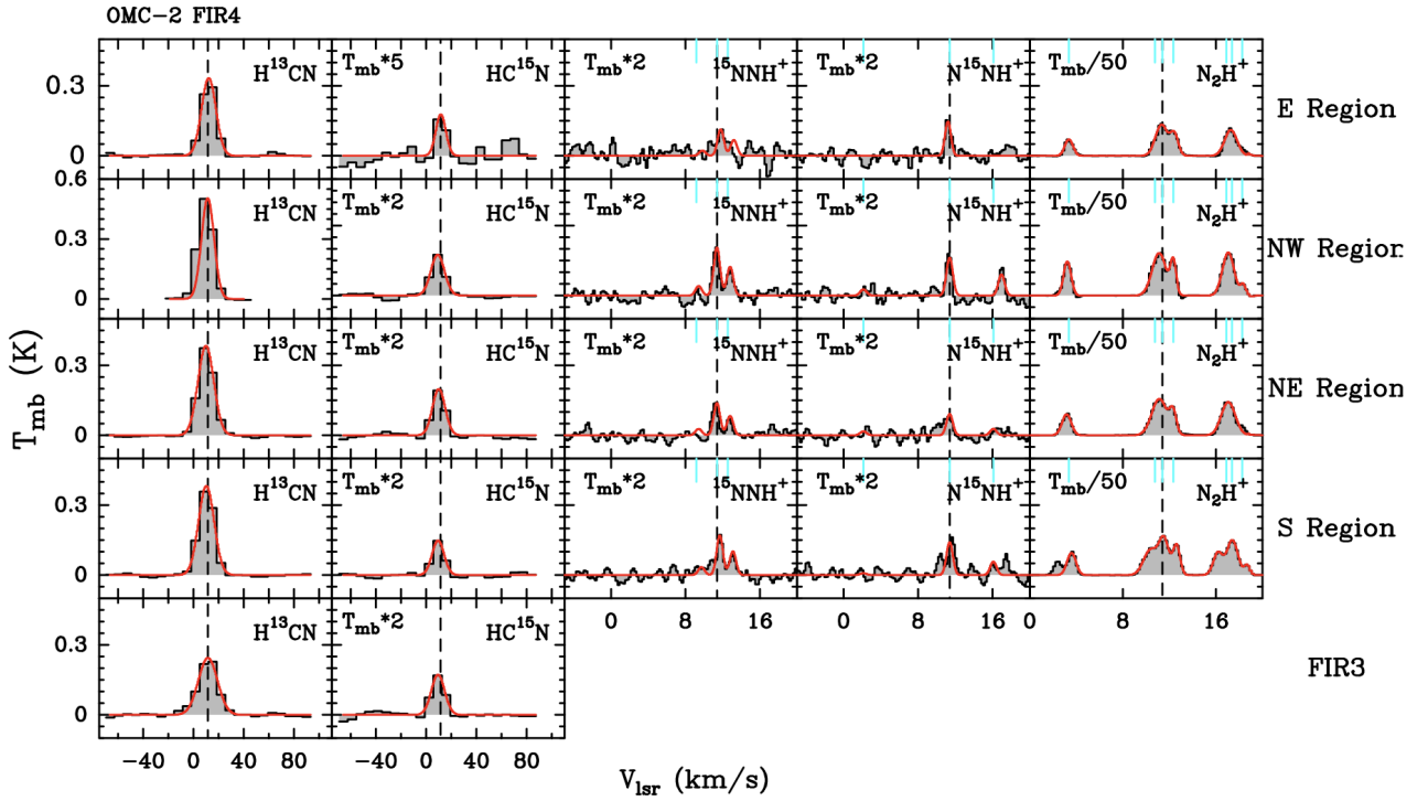
Fig. A.1. Spectra extracted for our study in (left to right) H 13 CN (1 – 0), HC 15 N (1 – 0), 15 NNH + (1 – 0), N 15 NH + (1 – 0) and N 2 H + (1 – 0); from top to bottom, the spectra extracted in the E, NW, NE, S and FIR3 regions. The CASSIS fits are superimposed in red. The dashed black line represents the V_{\text{LSR}} value for this source, which is 11.4 km s -1 . The blue lines represent the location of the HFS components for N 2 H + and its 15 N isotopologues.
