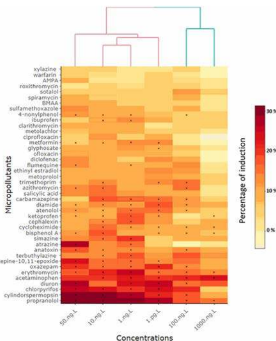
Fig. 2. Heatmap representing the luminescence variation between each micropollutant and the negative control based on the concentration tested. The gradation scale from yellow to red gives the percentage of induction, with luminescence variations of up to 30%. Clustering link was plotted using Euclidean distance method and Ward clustering linkage. Significant luminescence variations are indicated by a star. (For interpretation of the references to color in this figure legend, the reader is referred to the Web version of this article.)
