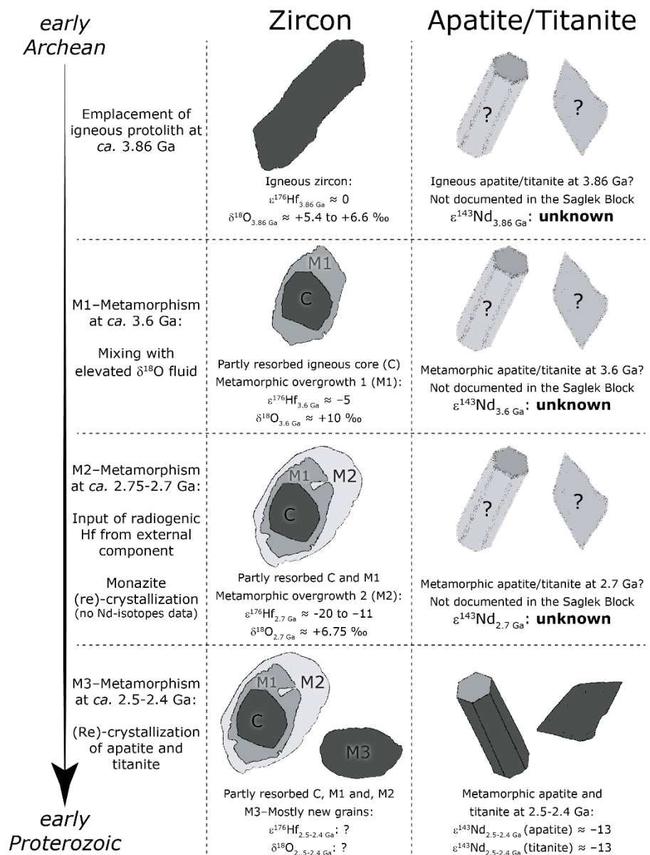
Figure 7. Evolution of Hf- and Nd-isotopes compositions of zircon and REE-rich minerals throughout the metamorphic history of the Archean Saglek Block.
