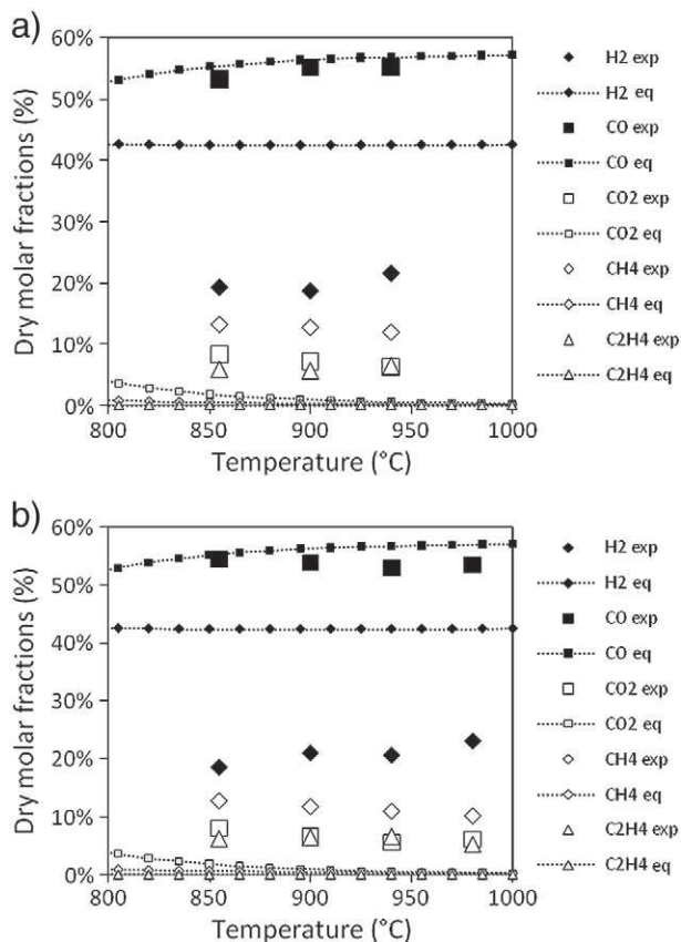
Fig. 12. Pyrolysis gases dry molar fractions vs temperature (X1 and S1). a) Oak, b) Fir.
