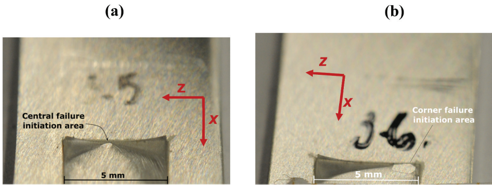
Figure 9. Typical failure initiation areas –(a) central failure initiation, (b) corner failure initiation.
