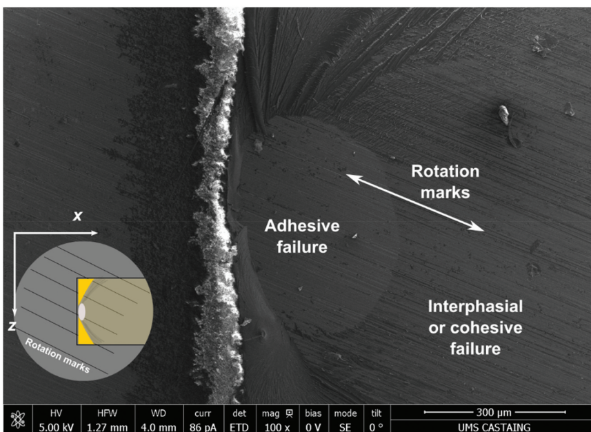
Figure 12. SEM of adhesive failure initiation –P1200.
