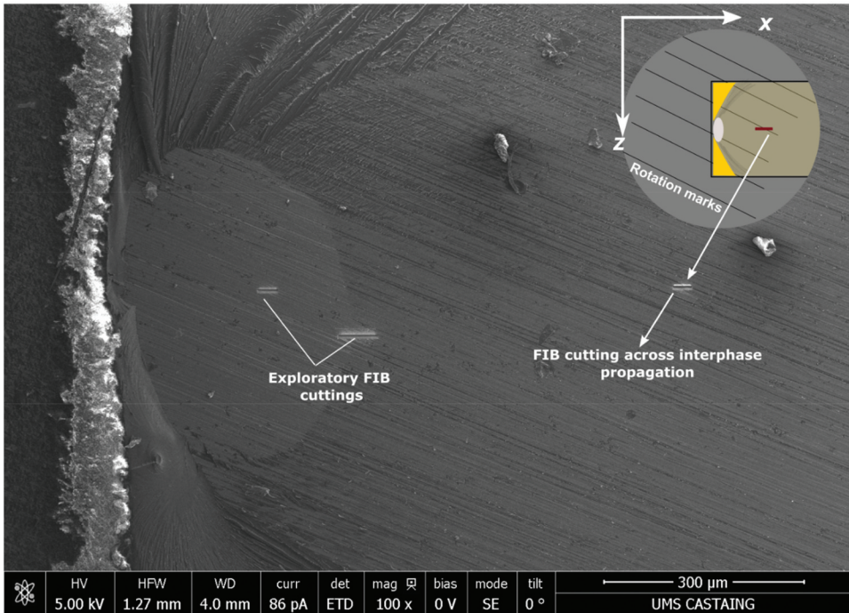
Figure 16. SEM of an interphasial failure propagation–FIB cutting is performed across interphase (on the right side).
