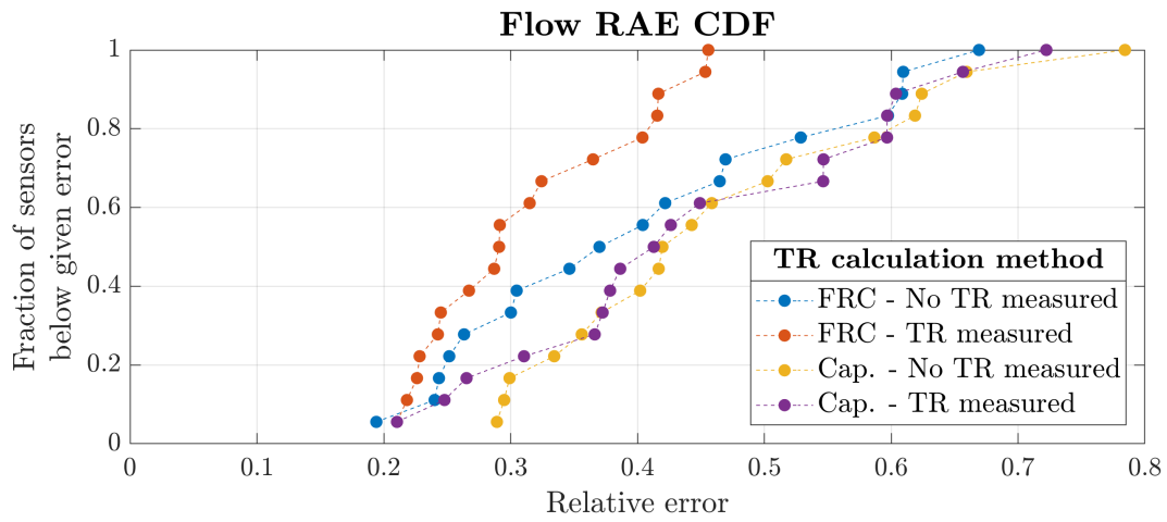
Figure 15: Relative estimation error CDF for the validation sensors using different TR values.
