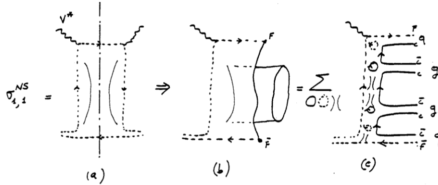
Fig. 22 -Cross section for cutting 1 reggeon and 1 pomeron in the non-singlet structure function: (a) cutting one pomeron and one reggeon; (b) produced string configuration: one mesonic open string plus one closed string; (c) interpretation as exclusive parton production cross section. All internal color loops, flavor loops and handles are summed over.
