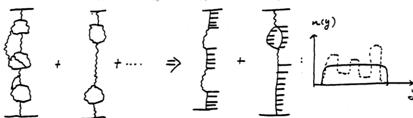
Fig. 17 - Fluctuating multiplicity distribution expected for \alpha_0 = 1
