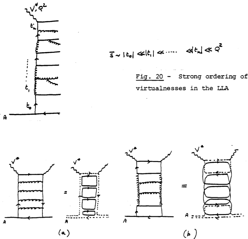
Fig. 21 - Topologies of the generalized latter diagrams in the LLA
