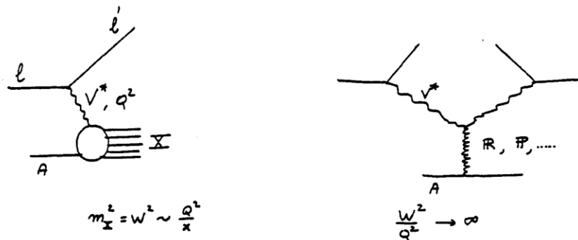
Fig. 19 - Regge model in DIS ( V^* is a \gamma^* , W^* or Z^* according to the type of leptons)
