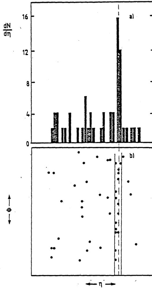
Fig. 26 - UA5 observation of a ring like event.
