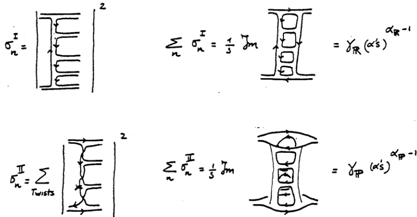
Fig. 8 - Building the planar reggeon \alpha_R and cylindrical pomeron \alpha_P from
