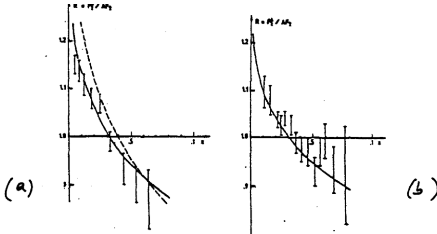
Fig. 25 - Estimate of the EMC affect - ref. [16] (a) full line: iron compared to data - dotted line prediction for uranium; (b). aluminium compared to data
