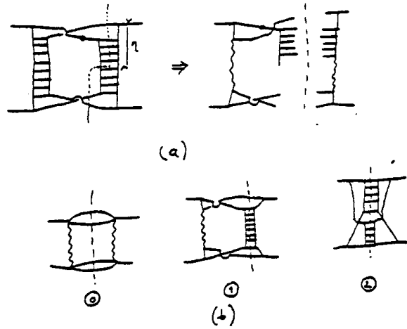
Fig. 14 (a) cutting leading to a vanishing absorptive part; (b) the three cuttings leading to non vanishing absorptive parts: none cut reggeon, one cut reggeon and two cut reggeons.
