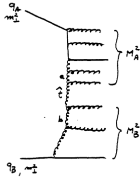
Fig. 24 - The LLA q_A q_B cross section with a gluon exchange with virtualness \hat{t} .
