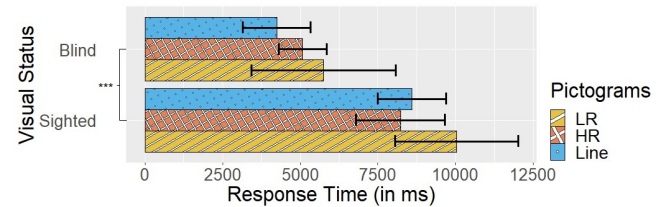
Fig. 2. Effect of illustration condition and visual status on response time: Mean response time and confidence interval (95%)
