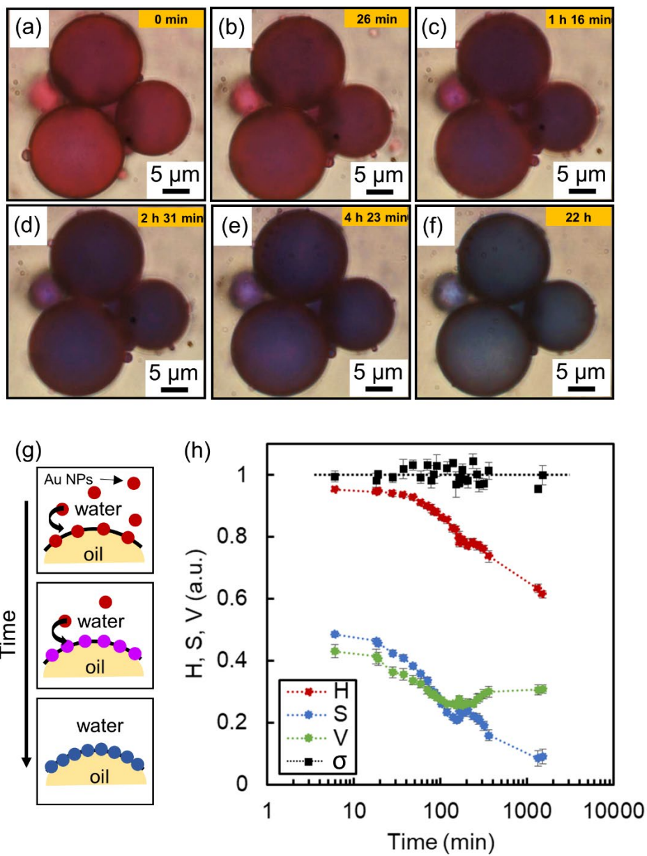
Figure 3. (a-f) Color change of the droplets due to the adsorption of Au NPs as a function of time. (g) Schematic representation of Au NPs adsorption at the oil/water interface over time and consequent change of color of the droplets. (h) Hue, saturation, value (H, S and V respectively - dots) and \sigma -radius of oil droplets normalized by the radius of oil droplets at 0 min (squares) as a function of time (values were averaged on 5 oil droplets).
