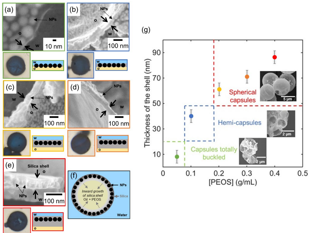
Figure 5. (a-e) SEM images of the shell of the Au-Si MCs obtained with (a) 0.05, (b) 0.1, (c) 0.2, (d) 0.3 and (e) 0.4 g/mL of PEOS. The oil phase “o” is toluene, the aqueous phase “w” is
