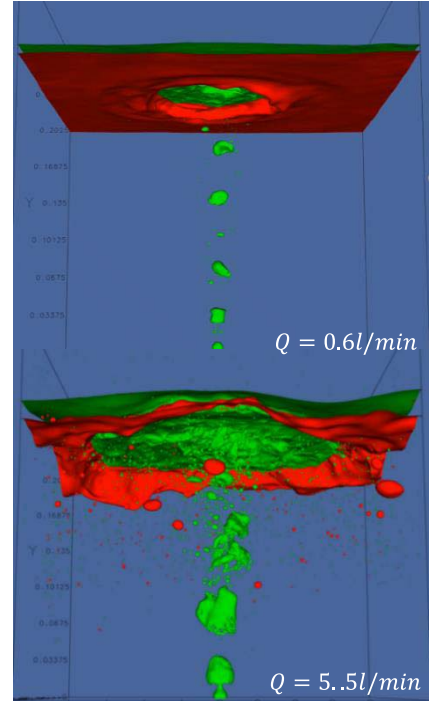
Fig. 6. Front view of the simulation with d_{inj} = 7.9\ \text{mm} with a minimum grid size \Delta_{min} = 527\ \mu\text{m} . The air interface is colored in green, and the oil interface is colored in red.
