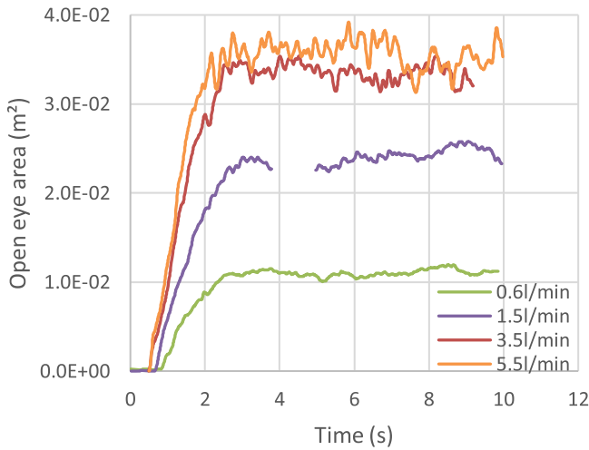
Fig. 5. Time evolution of the open eye area for different air flow rates with d_{inj} = 7.9\ \text{mm} . The results are obtained with a minimum grid size \Delta_{min} = 527\ \mu\text{m} corresponding to a maxlevel = 9 of adaptive refinement.
