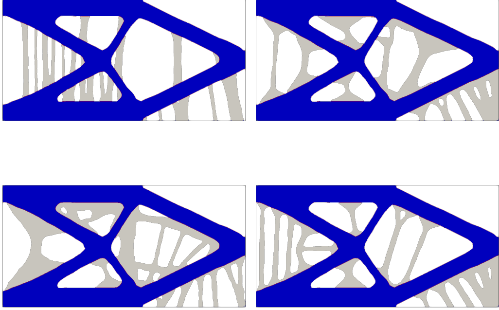
Figure 10: Optimized designs for \alpha = \beta = 0.001 (upper left), \alpha = \beta = 50 (upper right), \alpha = 10, \beta = 50 (lower left) and \alpha = 50, \beta = 10 (lower right).
