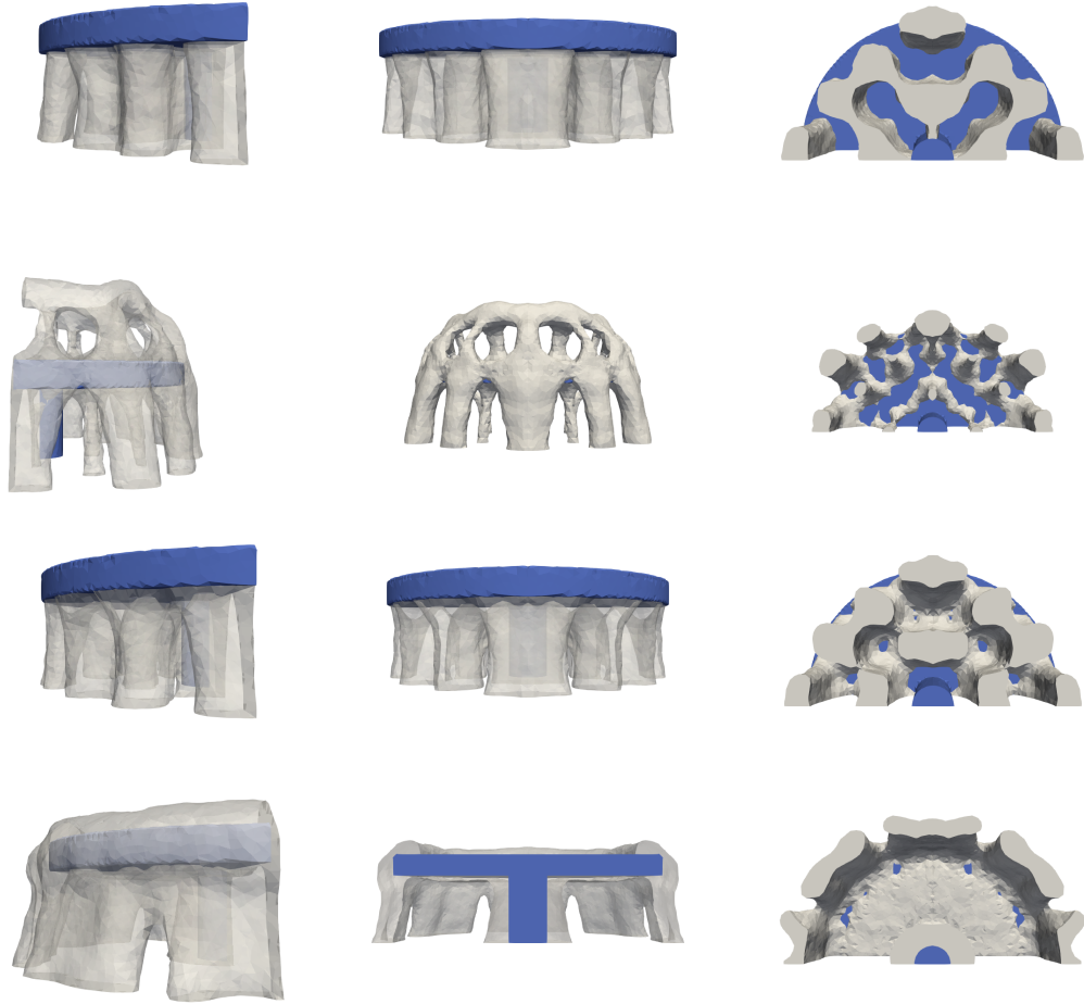
Figure 17: Different views of the optimized designs for the 3-d table: perfect interface (upper row), \alpha = \beta = 400 (2nd row), \alpha = 100, \beta = 1 (3rd row) and \alpha = 1, \beta = 100 (lower row).
