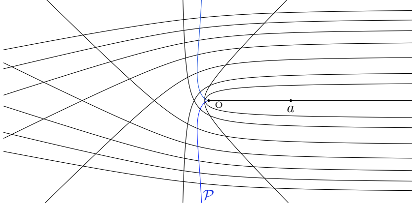
FIGURE 4. Hyperbolic motions of the Kepler problem with fixed value of the energy constant h > 0 and asymptotic velocity a in the future. All but one of these motions are bi-hyperbolic. The blue curve \mathcal{P} is composed of the corresponding perihelia.
