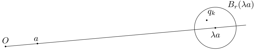
FIGURE 2. The C^1 approximation of the curve \gamma by h -minimizers from q_0 to q_k = p_{n_k} . Here \lambda = \lambda_{n_k} and \|q_k - \lambda a\| < r = o(\lambda) .
