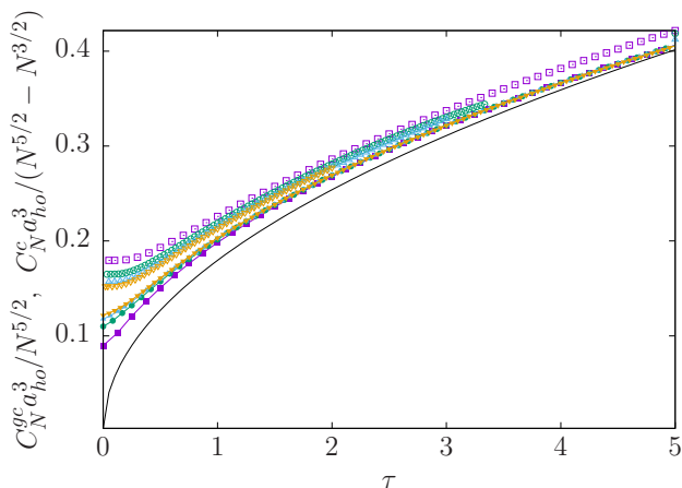
FIG. 6: Canonical (empty symbols) and grand-canonical contact (full symbols) as a function of \tau for N = 2 (violet squares), N = 3 (green circles), N = 4 (light-blue up-triangles), and N = 5 (orange down-triangles) Tonks-Girardeau bosons. The canonical contact [Eq. (7)] is rescaled by a factor N^{5/2} - N^{3/2} , while the grand-canonical one [Eqs. (8)-(9) in [46]] is rescaled by N^{5/2} . The black continuous curve corresponds to \sqrt{\tau}/\pi^{3/2} [Eq. (20)].
