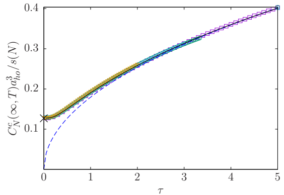
FIG. 3: Canonical contact in the Tonks-Girardeau limit C_N(\infty, T) , Eq. (7), as a function of \tau , scaled by the factor s(N) = N^{5/2} - N^{3/4(1+\exp(-2/\tau))} , see Eq. (23). Violet squares: N = 2 , green circles: N = 3 , light-blue up-triangles: N = 4 and orange down-triangles: N = 5 . The blue dashed line corresponds to the high-temperature limit h_2(\infty, \tau \gg 1) [Eq. (20)]. The black cross and the black line correspond to h_2(\infty, 0) = (2/\pi)^{3/2} a_{ho}^{-3} (2^{5/2} - 2^{3/4})^{-1} and h_2(\infty, \tau) [Eq.(24)] respectively.
