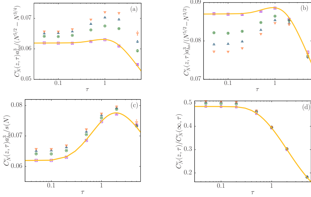
FIG. 4: Panels (a), (b) and (c): C_N^c(z, \tau) a_{ho}^3 as a function of \tau , for the case z = 1 , rescaled by N^{5/2} - N^{3/4} (a), N^{5/2} - N^{3/2} (b), and s(N) (c). Panel (d): f_N(z = 1, \tau) as a function of \tau . The points (violet squares: N = 2 , green circles: N = 3 , light-blue up-triangles: N = 4 and orange down-triangles: N = 5 ) correspond to the QMC data. The continuous yellow line corresponds to the two-bosons contact obtained by Eq. (5). Non visible QMC error bars are smaller than the symbol size.
