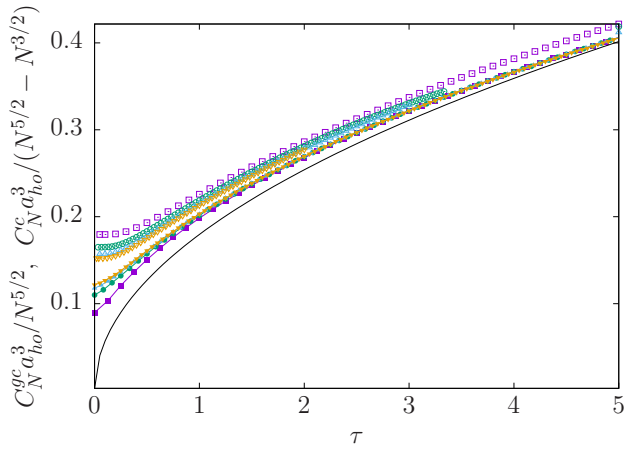
FIG. 6: Canonical (empty symbols) and grand-canonical contact (full symbols) as a function of \tau for N = 2 (violet squares), N = 3 (green circles), N = 4 (light-blue up-triangles), and N = 5 (orange down-triangles) Tonks-Girardeau bosons. The canonical contact [Eq. (7)] is rescaled by a factor N^{5/2} - N^{3/2} , while the grand-canonical one [Eqs. (8)-(9) in [46]] is rescaled by N^{5/2} . The black continuous curve corresponds to \sqrt{\tau}/\pi^{3/2} [Eq. (20)].
