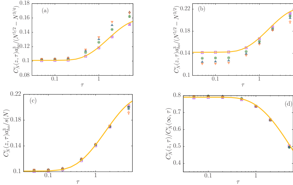
FIG. 5: Panels (a), (b) and (c): C_N^c(z, \tau) a_{ho}^3 as a function of \tau , for the case z = 2.5 , rescaled by N^{5/2} - N^{3/4} (a), N^{5/2} - N^{3/2} (b), and s(N) (c). Panel (d): f_N(z = 2.5, \tau) as a function of \tau . The points (violet squares: N = 2 , green circles: N = 3 , light-blue up-triangles: N = 4 and orange down-triangles: N = 5 ) correspond to the QMC data. The continuous yellow line corresponds to the two-bosons contact obtained by Eq. (5). Non visible QMC error bars are smaller than the symbol size.
