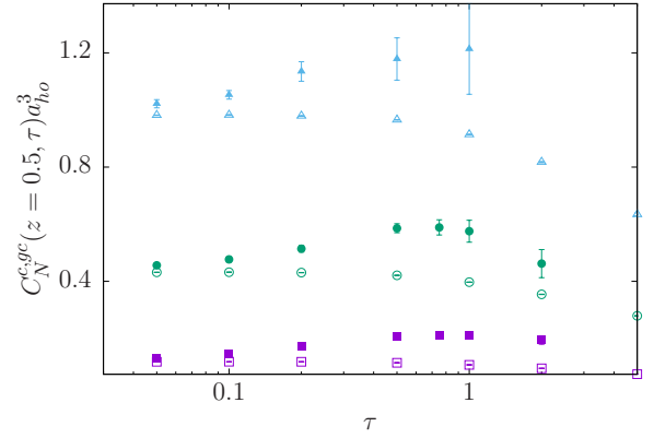
FIG. 7: Canonical (empty symbols) and grand-canonical contact (full symbols) as a function of \tau for N = 2 (violet squares), N = 3 (green circles), N = 4 (light-blue up-triangles) bosons. All points correspond to QMC data evaluated in the weakly-interacting regime z = 0.5 . QMC error bars for the canonical data are smaller than the symbol size.
