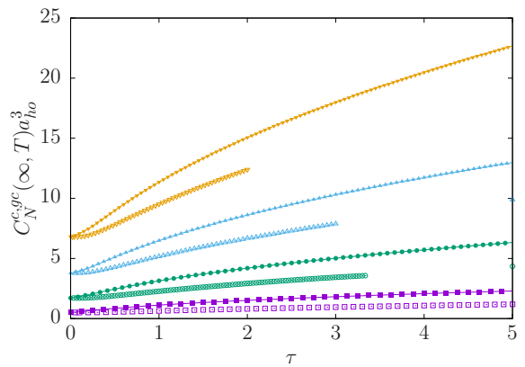
FIG. 2: Canonical (empty symbols) [Eq. (7)] and grand-canonical contact (full symbols) [46] as a function of \tau for N = 2 (violet squares), N = 3 (green circles), N = 4 (light-blue up-triangles), and N = 5 (orange down-triangles) Tonks-Girardeau bosons. The grand-canonical case will be discussed in Sec. IV.
