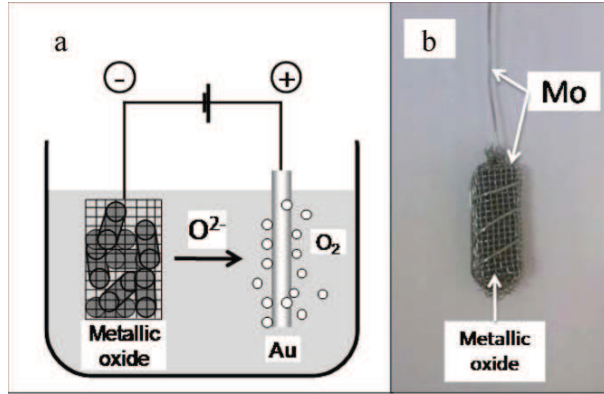
Fig. 1. (a) Schematic representation of the FFC Cambridge process and (b) picture of metallic oxide sample.
