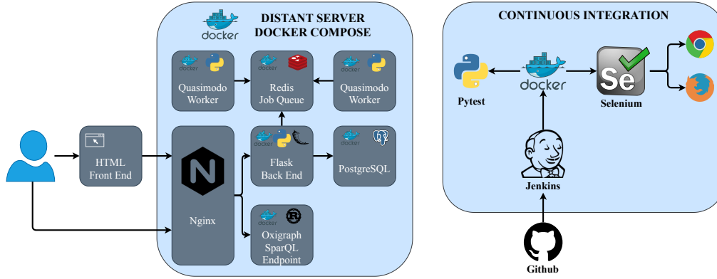
Figure 2: The web portal architecture.
