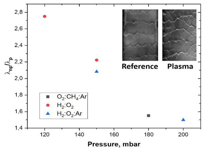
Figure 2. Measured cell sizes against initial pressure
